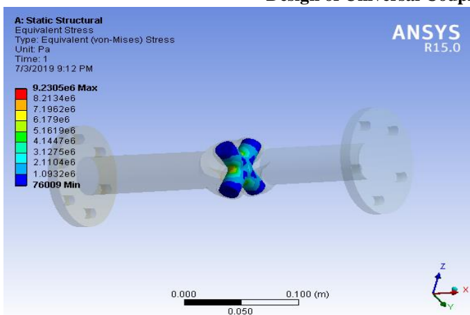
Fig.4 Equivalent Von-Mises Stresses in spider
