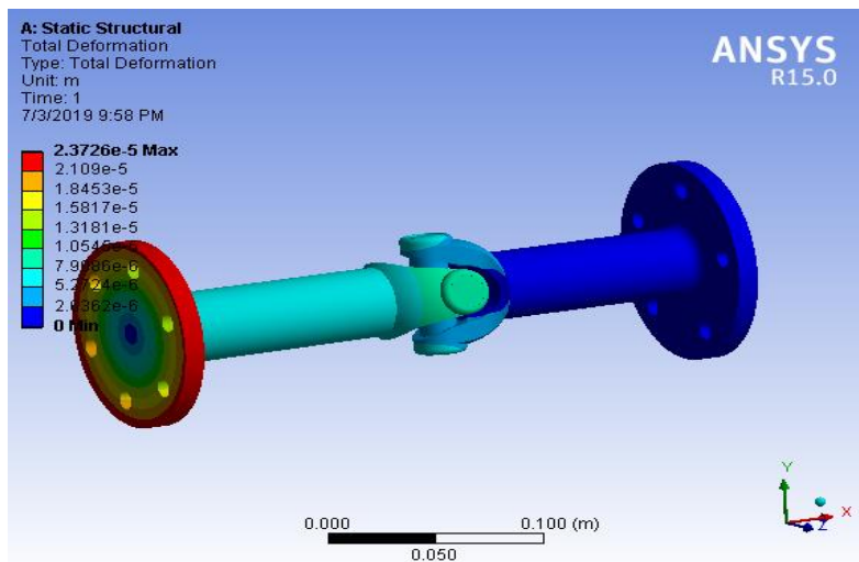
Fig.13 Total deformation in universal joint analyzed using Grey Cast Iron material
