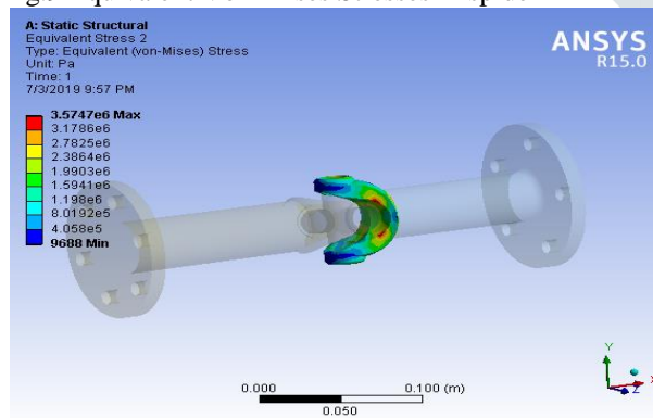
Fig.9 Equivalent Von-Mises Stresses in spider
