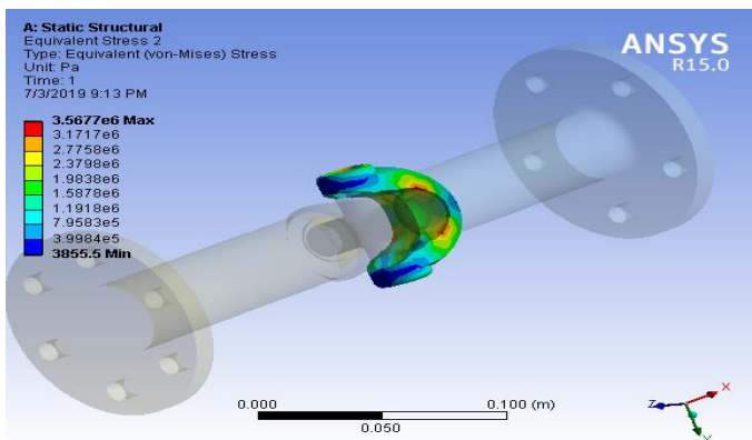
Fig.6 Equivalent Von-Mises Stresses in driven yoke
