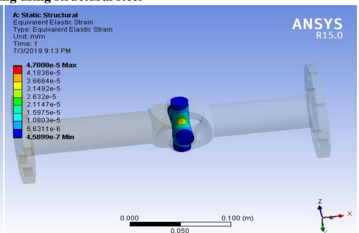
Fig.5 Equivalent Elastic Strain in spider
