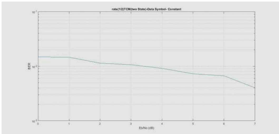
Fig. 3: BER Graph of 1x2 TCM Encoded OFDM-IM Data Symbol Constant
