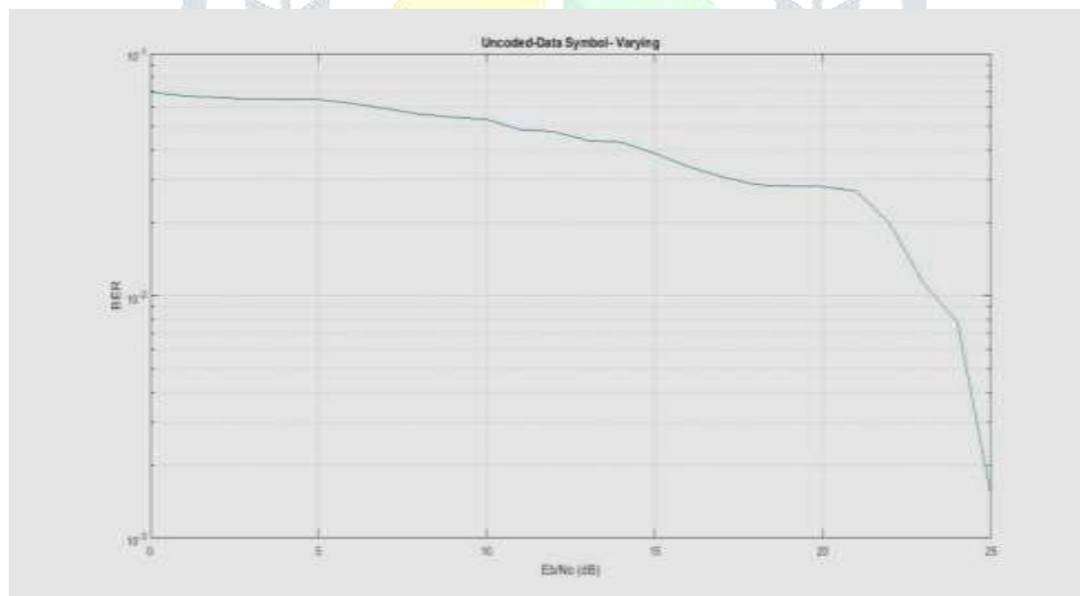
Fig. 4: BER Graph of Uncoded OFDM-IM Data Symbol Varying
