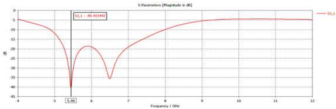
Figure 5: Return loss
