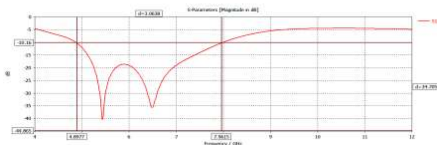
Figure 11: Bandwidth
