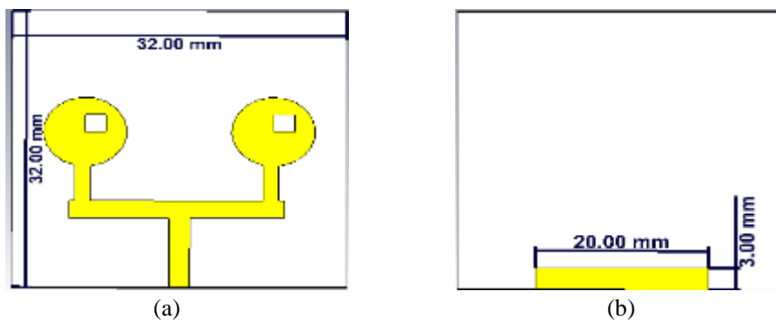
Figure 3: (a) Top view (b) Defected Ground Structure of proposed microstrip array antenna
