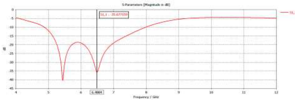
Figure 8: Return loss
