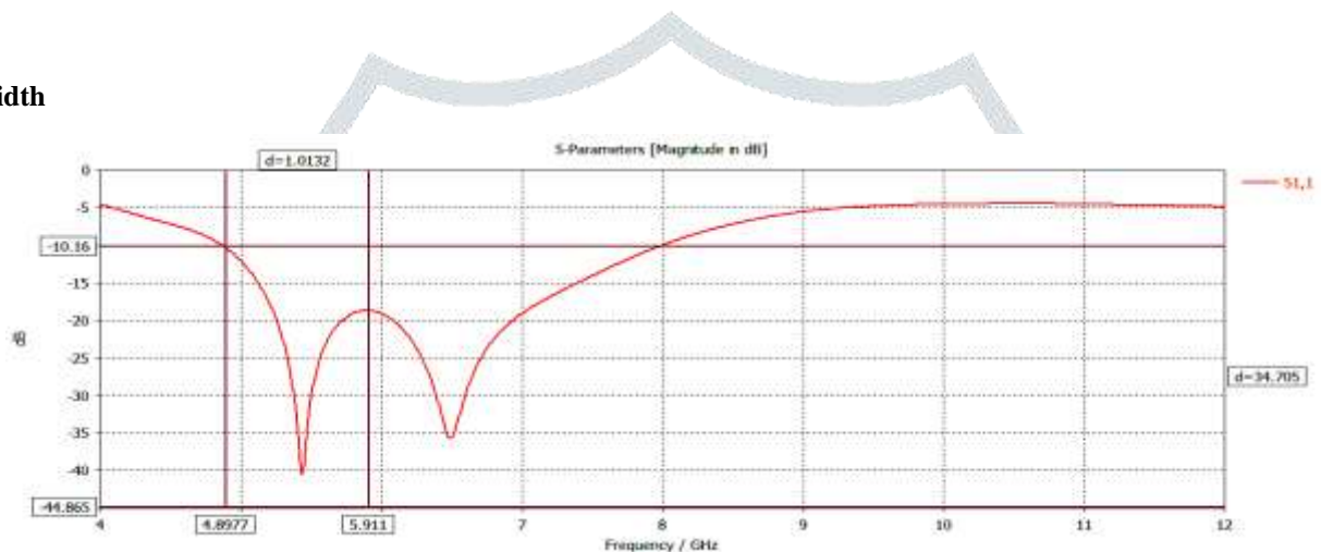
Figure 6: Bandwidth
