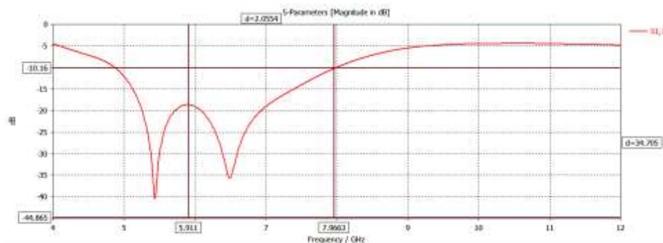
Figure 9: Bandwidth
