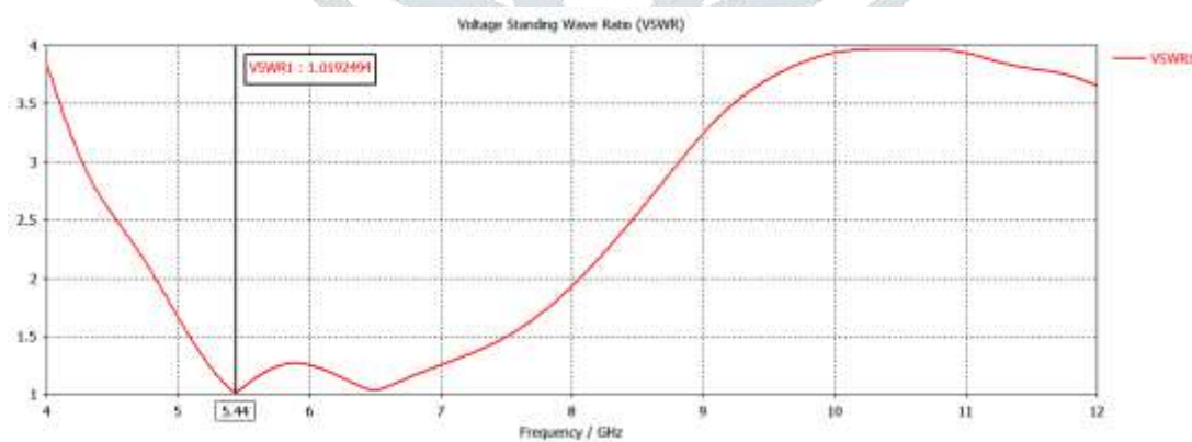
Figure 7: VSWR
