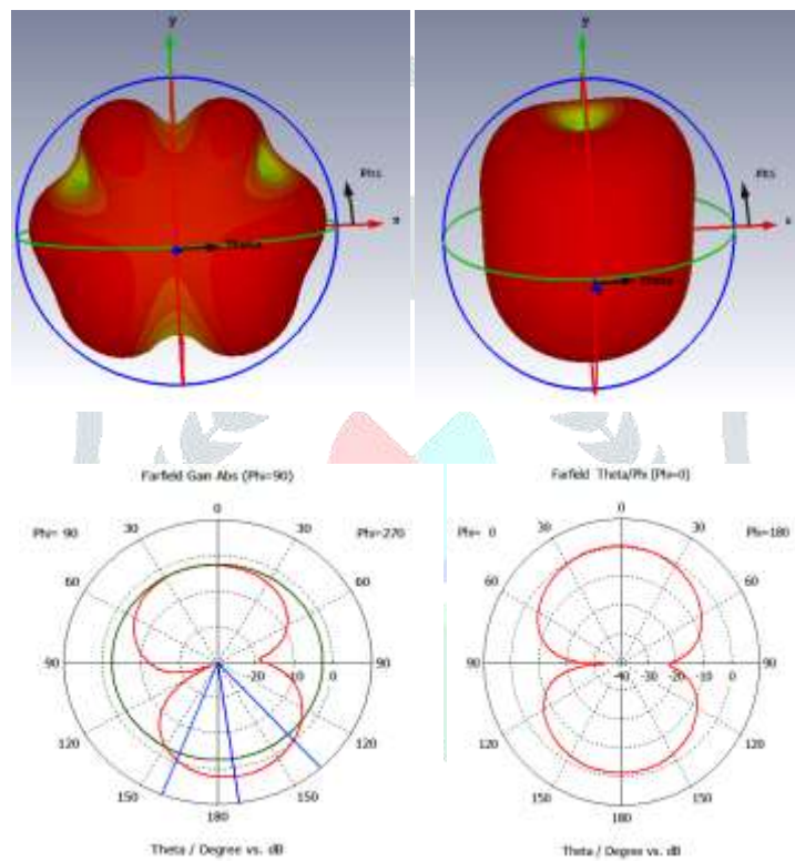
Figure 13: Radiation pattern
