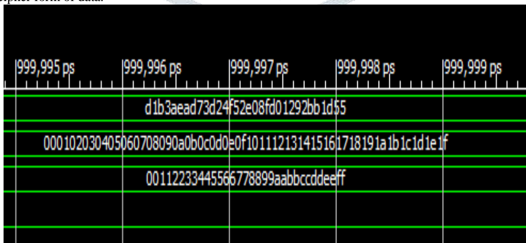
Figure 6: Decryption Process
