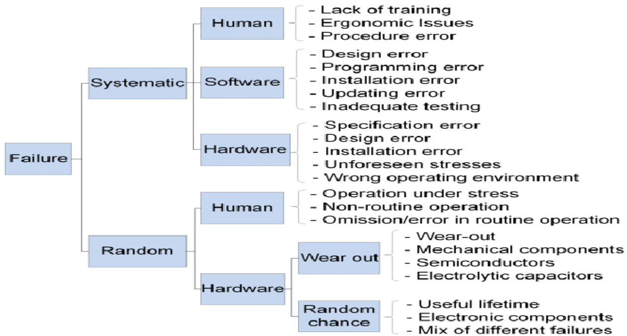
Fig. 1. Failures classification based on failure causes (sources)
