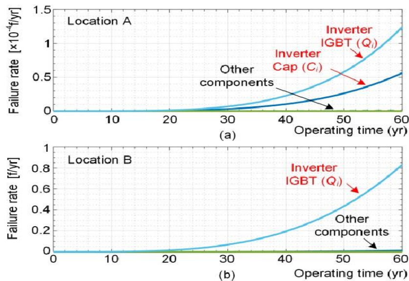
Fig. 6. Wear-out failure rate of individual components of converter under the mission profile of (a) Location A and (b) Location B.
