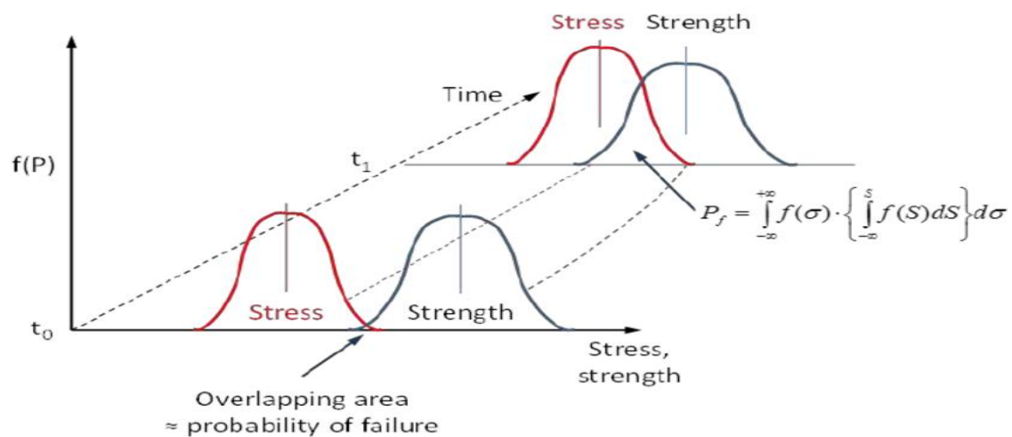
Fig. 2. Probability of failure estimation concept based on mismatch of stress and strength
