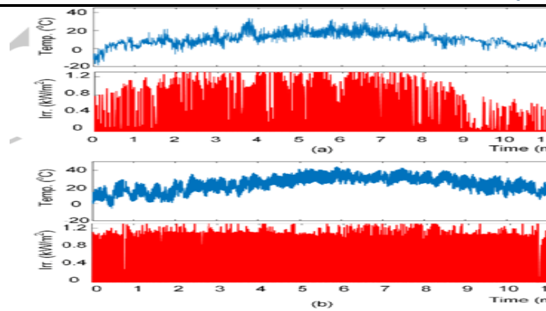
Fig. 5. Annual solar irradiance and ambient temperature for (a) Location A, (b) Location B
