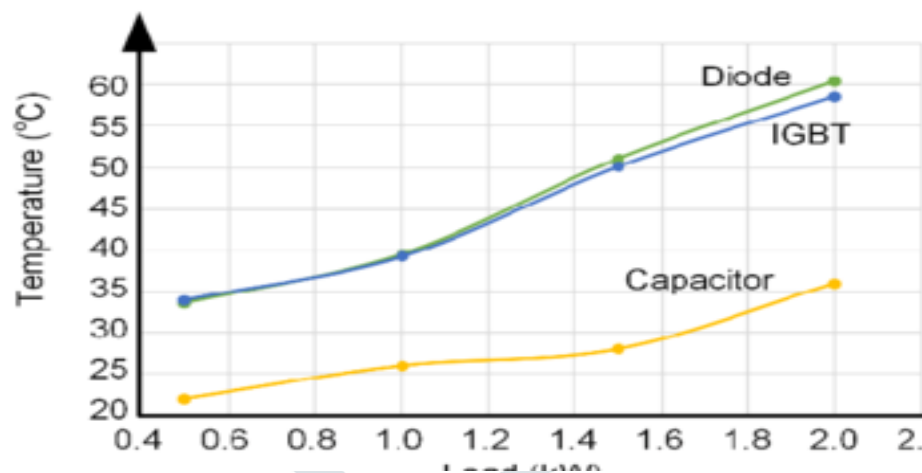
Fig. 4. Experimental results of boost converter; the IGBT, diode and capacitor temperatures under different loading conditions.
