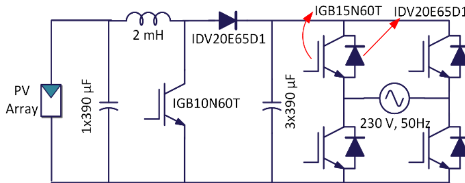
Fig. 3. Structure of the single-phase double-stage PV inverter
