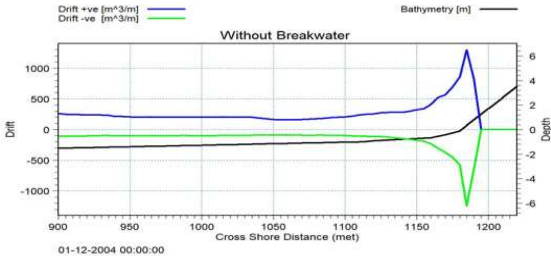
Fig. 10: Graph for littoral Drift without breakwater
