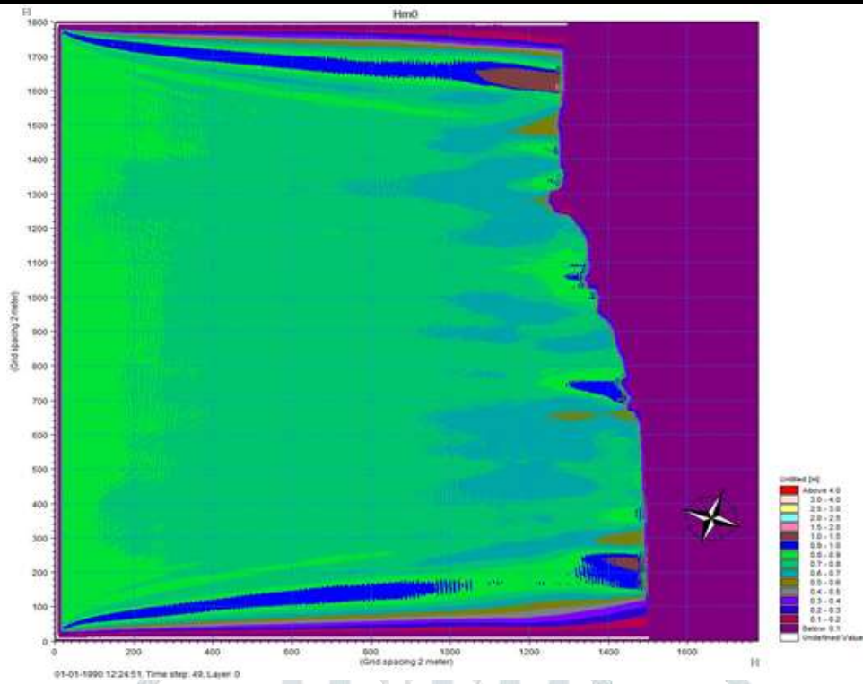
Fig.5: Significant wave height without permeable breakwater (WEC)
