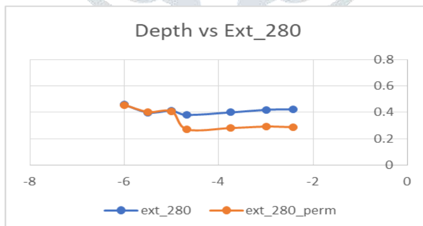
Fig 9: Graph between water depth Vs significant wave height for angle 280°, without the permeable breakwater (WEC) and with the permeable breakwater (WEC).
