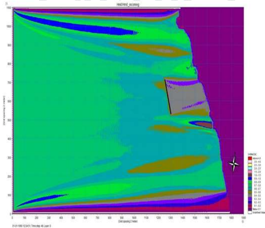
Fig. 6: Significant wave height with permeable breakwater (WEC) with angle of wave incidence 260°
