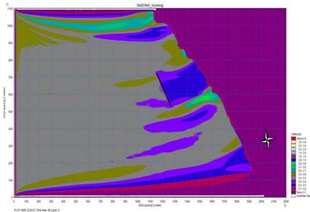
Fig. 8: Significant wave height with permeable breakwater (WEC) with angle of wave incidence 280°
