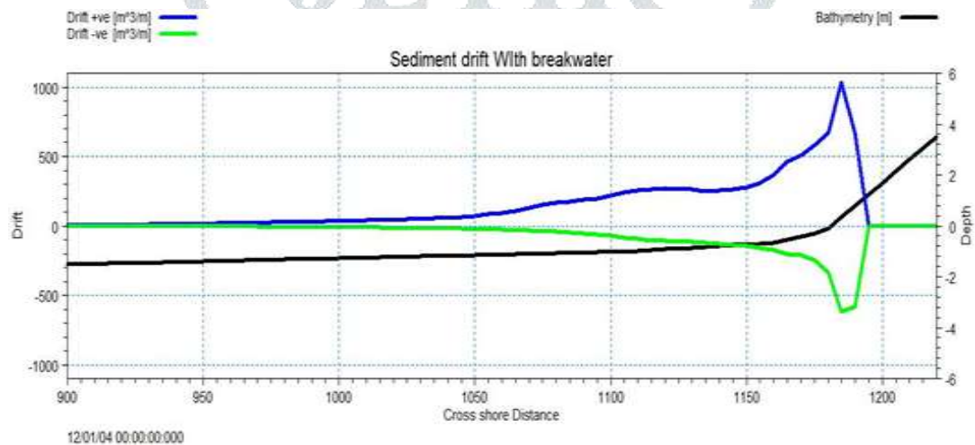
Fig. 11: Graph for littoral Drift with Breakwater.
