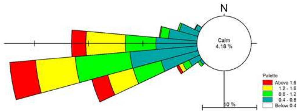
Fig. 3: Wave Rose Diagram obtain from SW model
