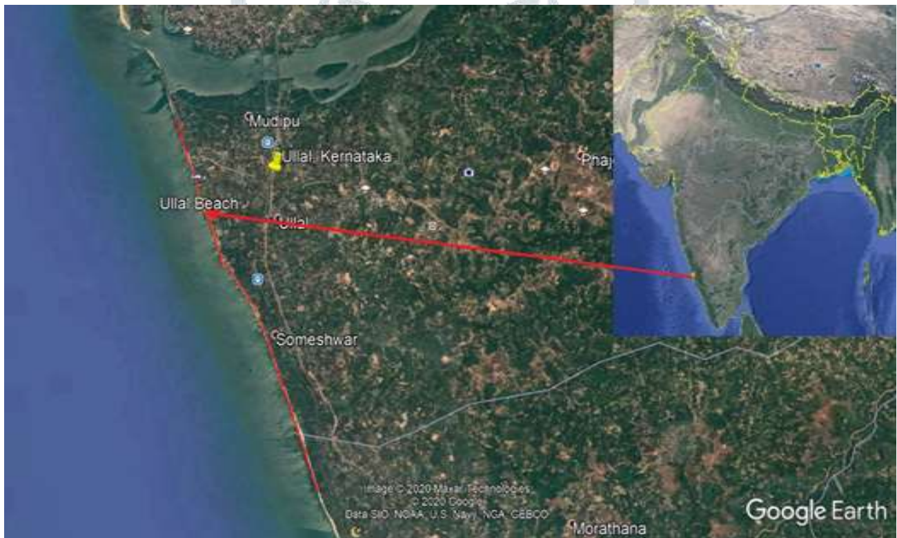
Fig. 1: Study Area
