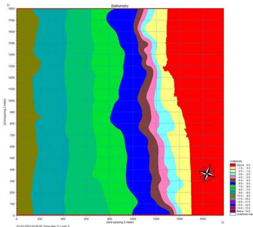
Fig. 2: Classical Bathymetry
