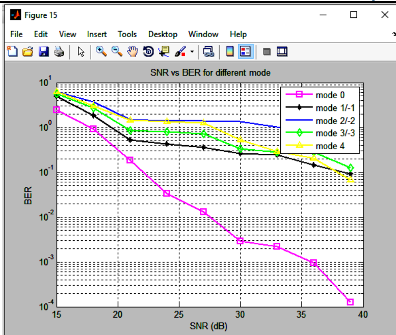
Figure 4: SNR vs BER for different OAM mode
