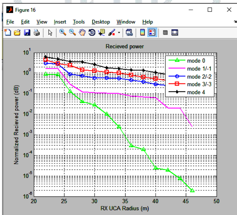
Figure 5: Received power
