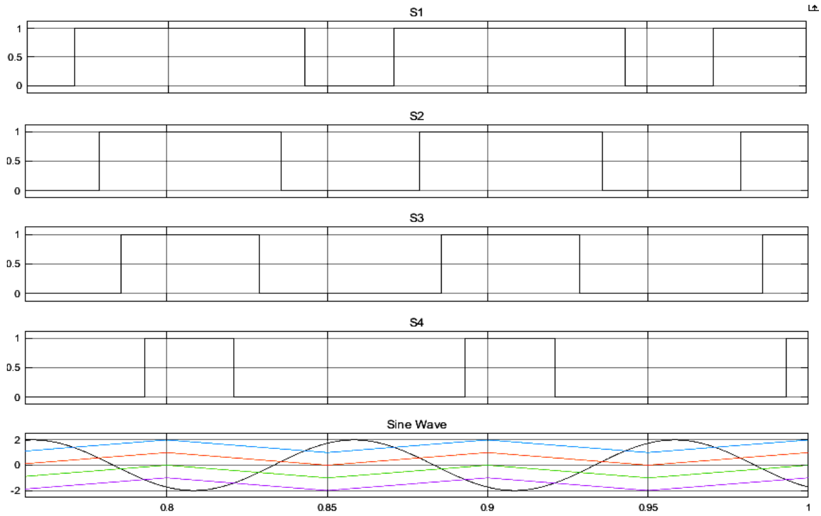
Figure 6: Switching Sequence shifted -120^\circ
