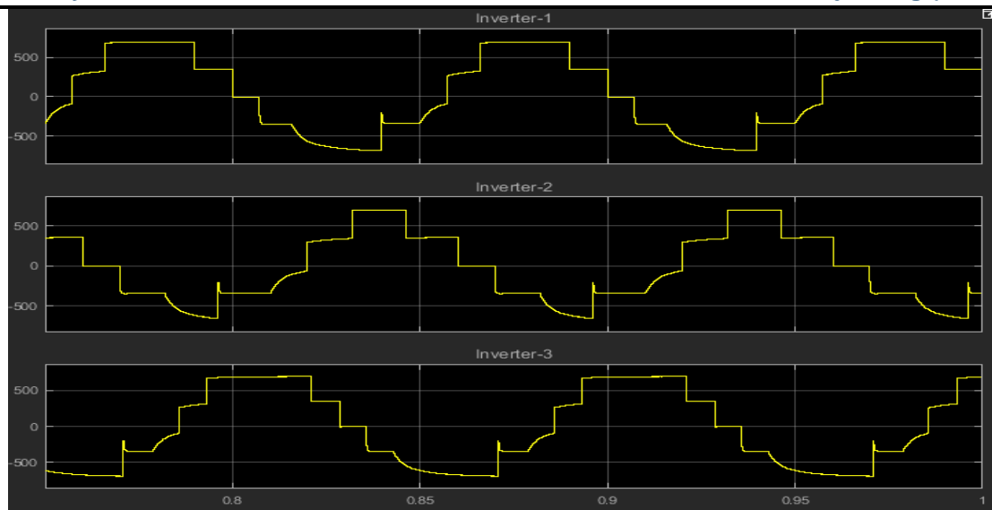
Figure 8: Inverter Voltage
