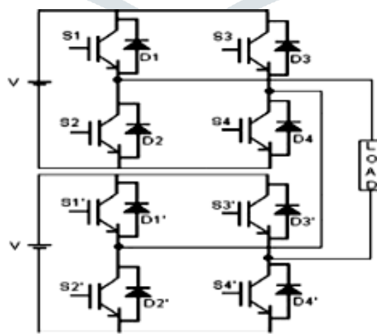
Figure 1: Five level Cascaded Inverter
