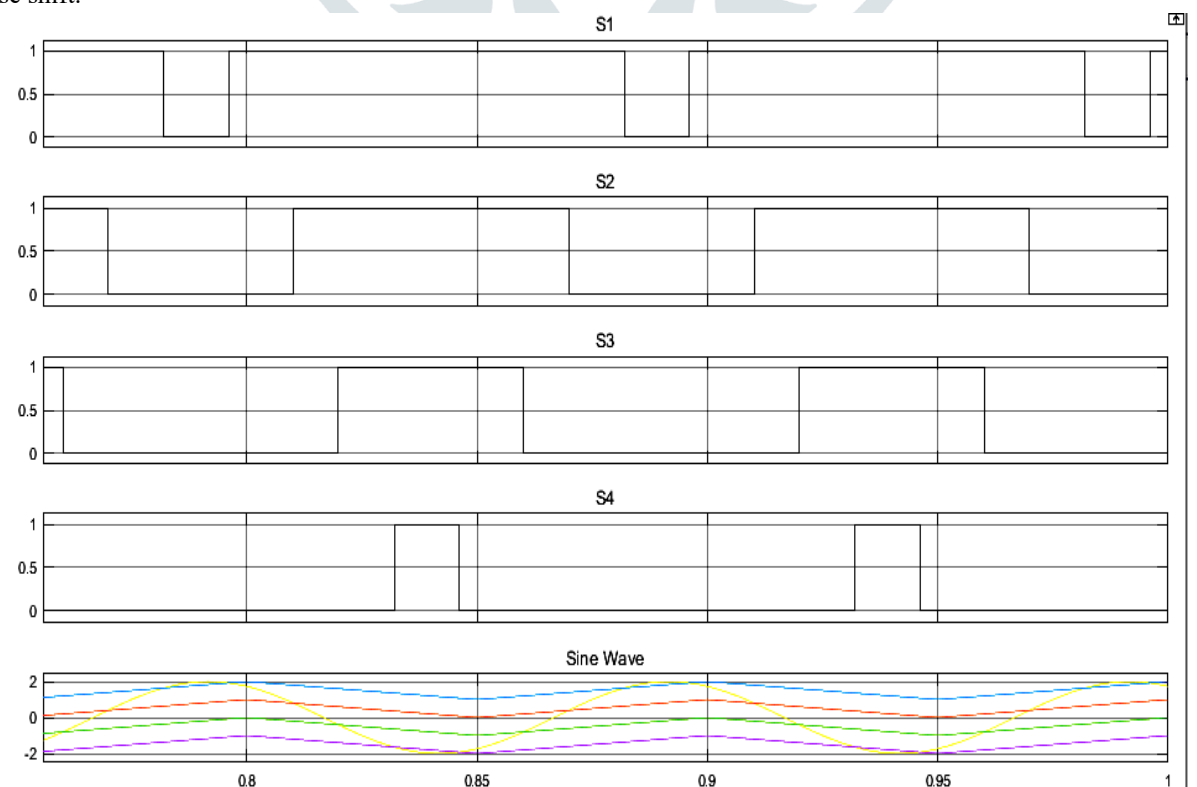
Figure 5: Switching Sequence shifted 120°
