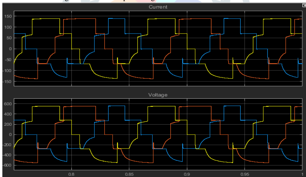
Figure 7: Inverter Output
