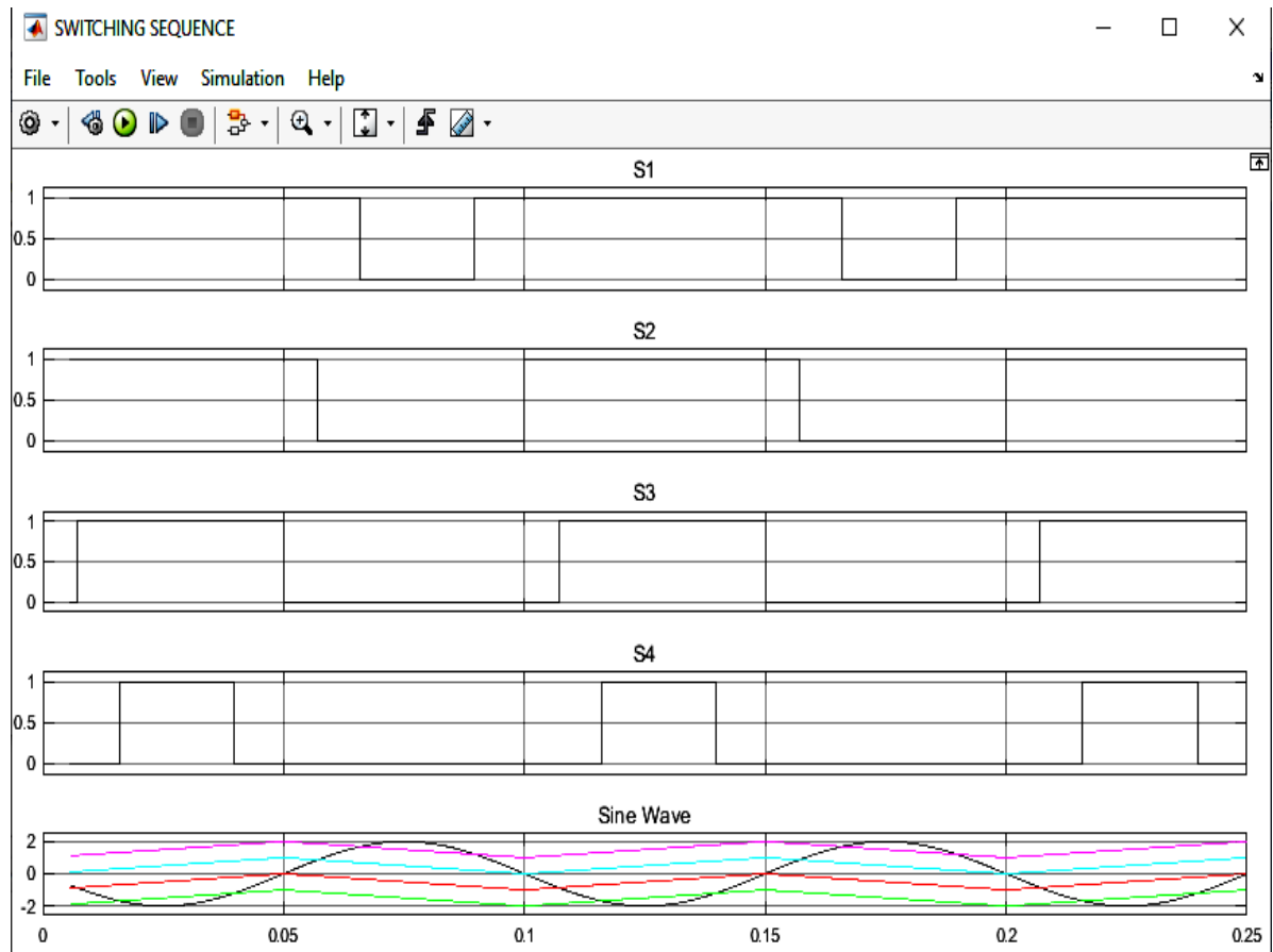
Figure 4: Switching Sequence
