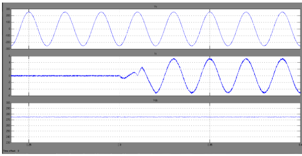
(a) PV array
