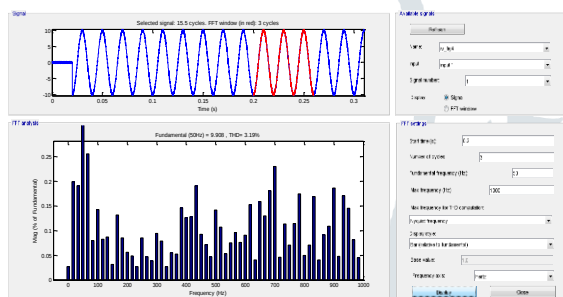
Total Harmonic Distortion (THD)
