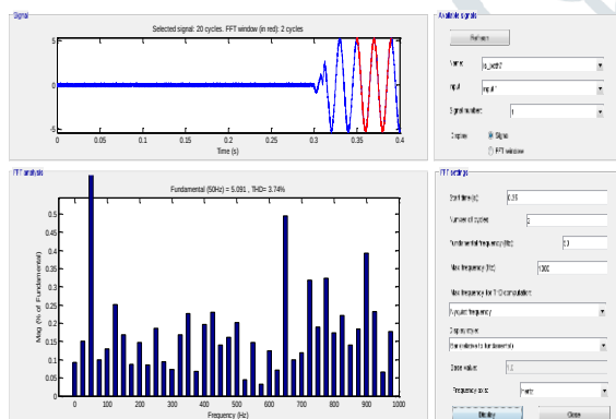
Total Harmonic Distortion (THD)
