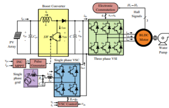
Fig.1 Schematic of the grid interactive PV array based water pumping system using a BLDC motor drive
