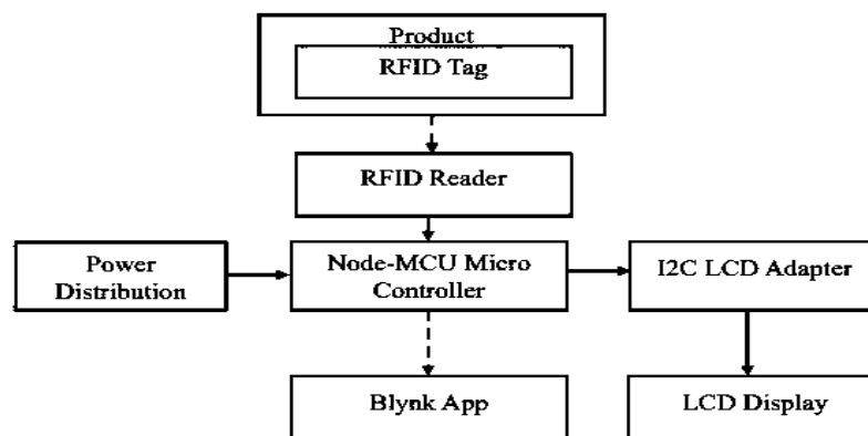
Block Diagram of proposed System
