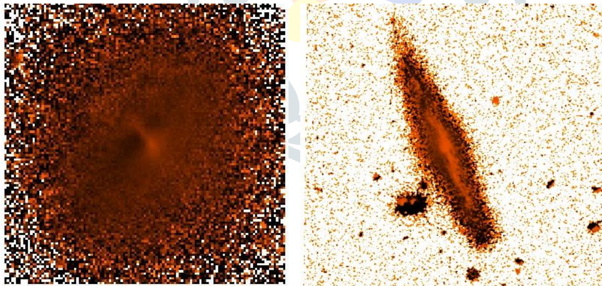
Figure 2: left panel image shows the (g - r) colour map of UGC 9519 galaxies and the right panel is the colour map of NGC 3696 galaxy.
