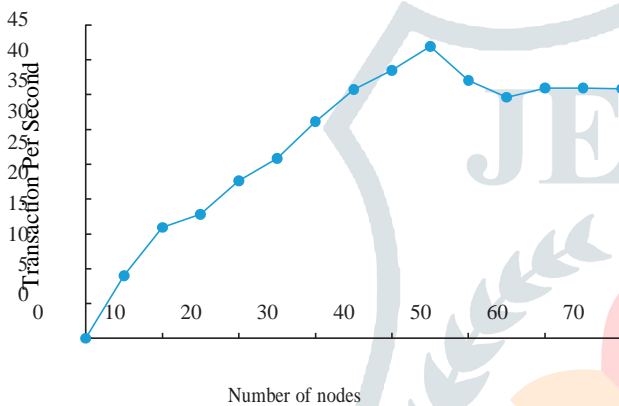
Figure 6: The throughput of the transaction system under different number of nodes.
