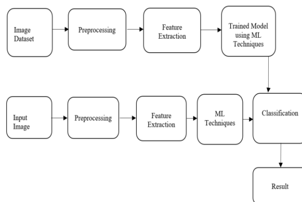
Fig 5 System Architecture
