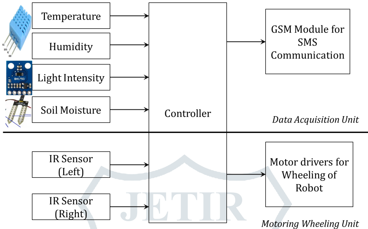
Figure 1: Block Diagram of Green House Monitoring Robot
