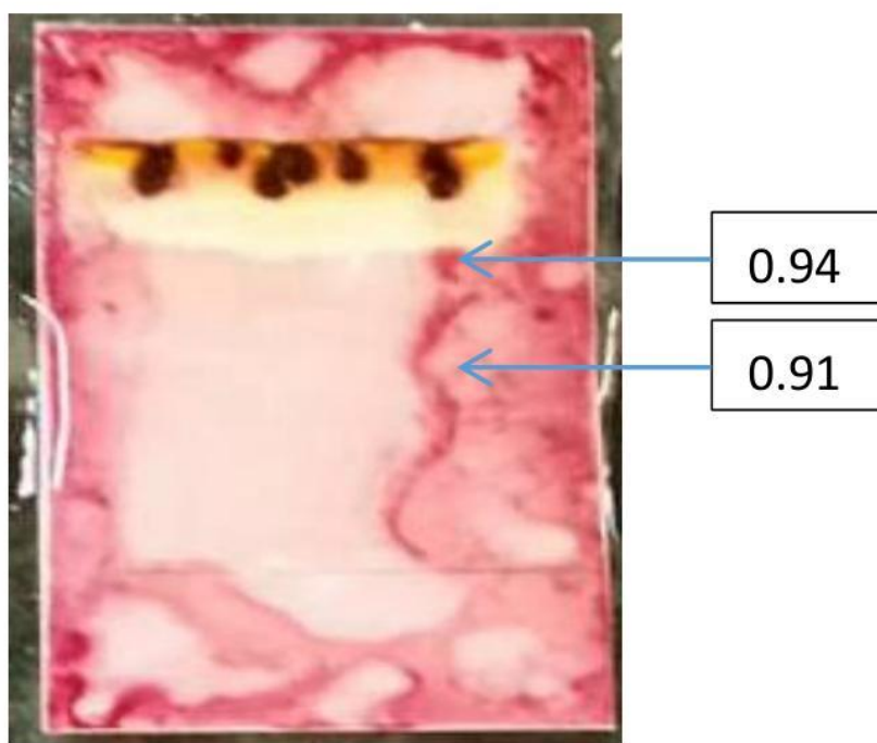
Fig. No. 21 TLC-bioautographic profile of D. senecioides acetate extracts against T. tonsurans [24]
