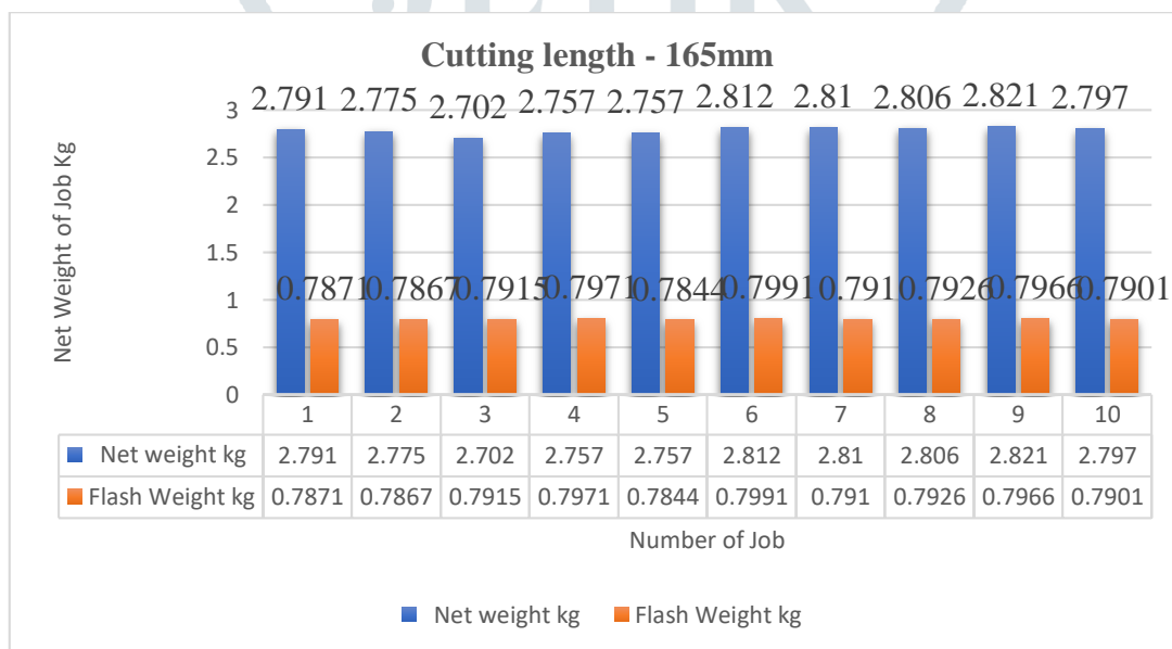
Fig 10 Relation Job Weight and Flash Weight
