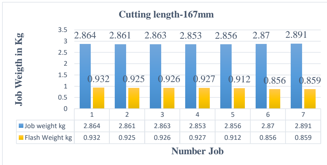
Fig 09 Relation Job Weight and Flash Weight
