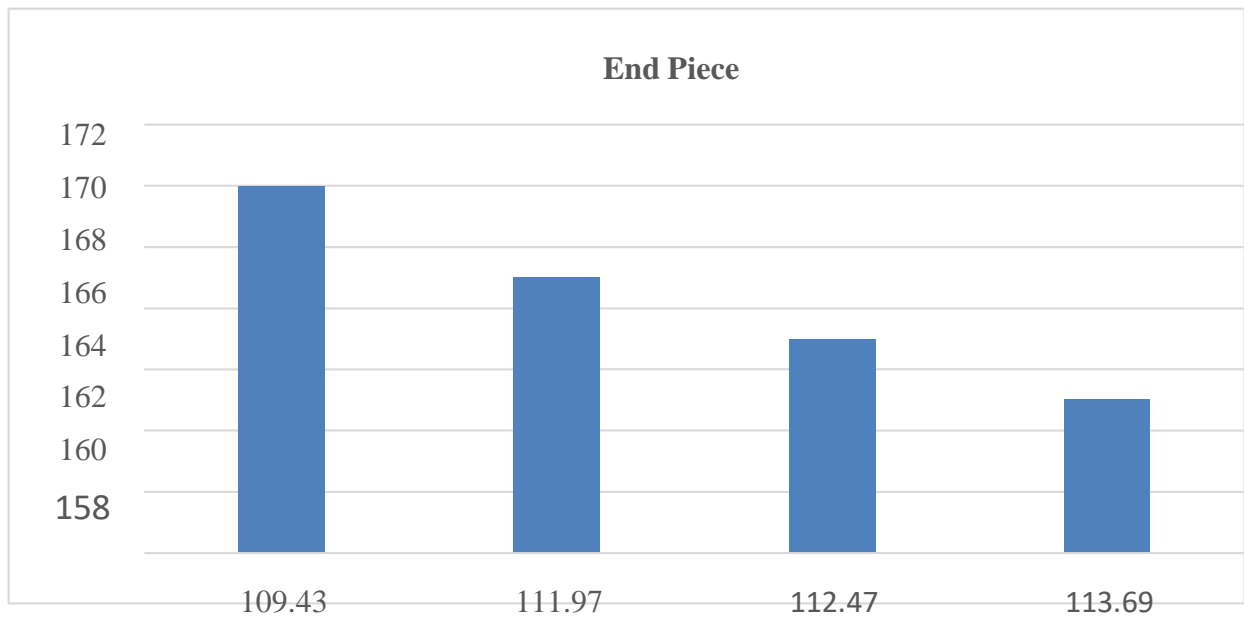
End pieces cutting length
