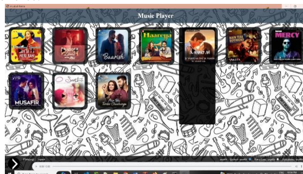
Fig. 3. Output screen
