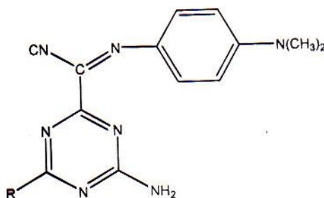
2,4-diamino-1,3,5-triazine
