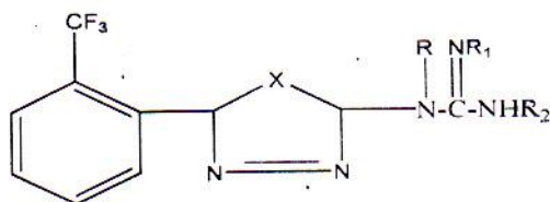
Substituted-1,3,4-thia/oxadiazoles
