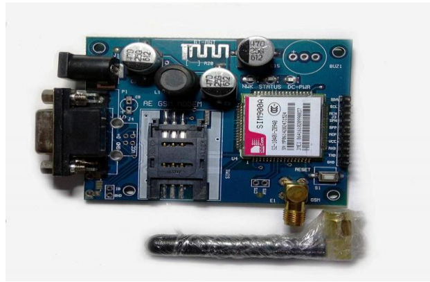
Figure 3: GSM 900A
