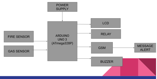
Fig 1:-flow chart
