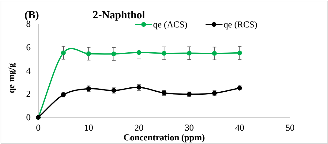
Figure 11: Effect of Initial Concentration on Uptake of PCs with both ACS and RCS Adsorbents. (Contact time: 30 min; shaking speed: 120 rpm; temperature: 25 ± 1 °C; pH: 5.0 for hydroquinone and pH 6.0 for 2-naphthol, 0.1 g dose).
