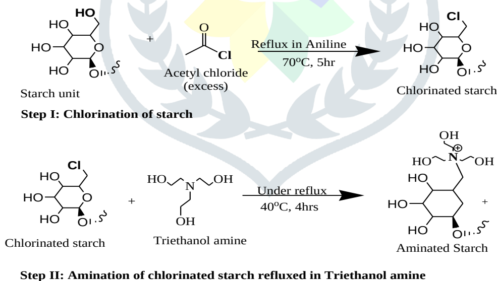
Scheme 3: The steps involved in Amination of dried cornstarch using triethanolamine [34].
