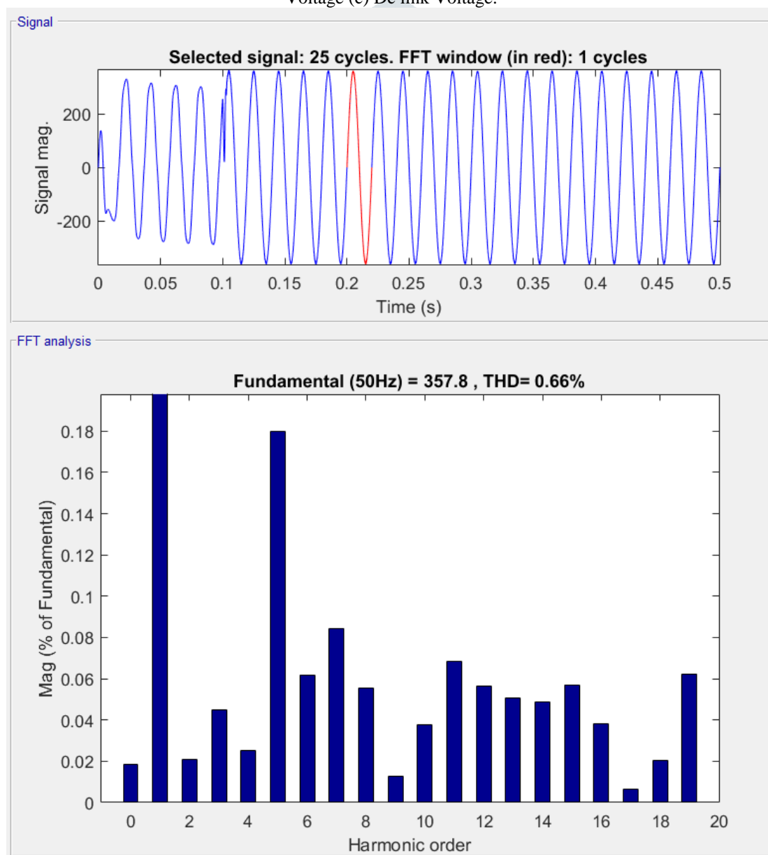
Fig9. Load Voltage THD% with the ANN controller Shunt Active filter
