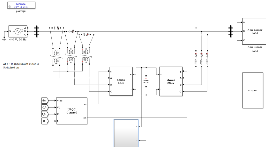
Fig5. Simulation Block Diagram of the Proposed System
