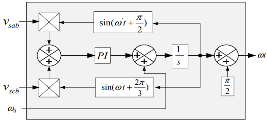
Fig.2 Improved PLL Scheme
