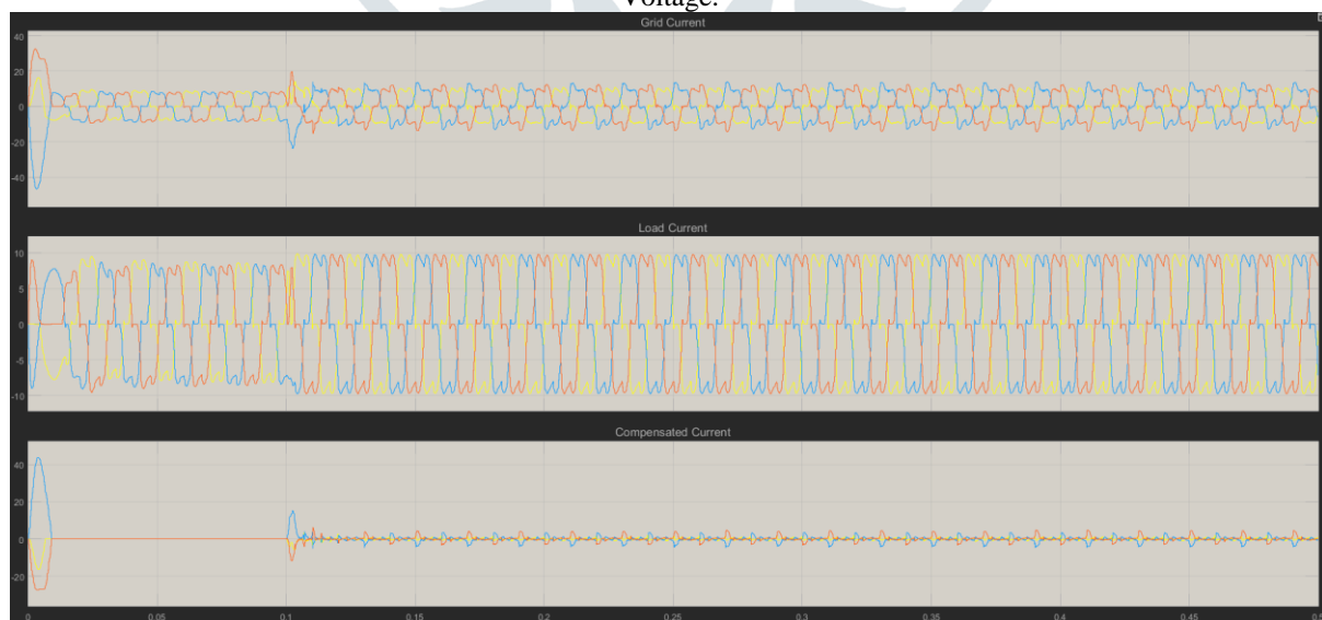
Figure7. Simulated waveforms of the proposed control scheme. (a) Phase to neutral source Current. (b) Load Current. (c) UPQC Current.
