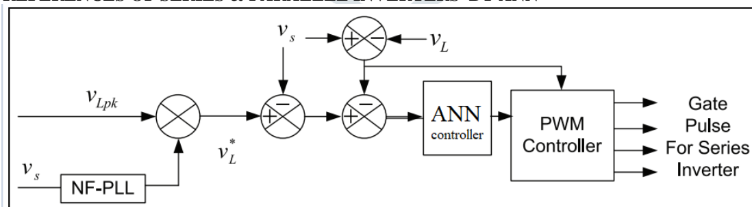
Figure 3. Control structure of ANN
