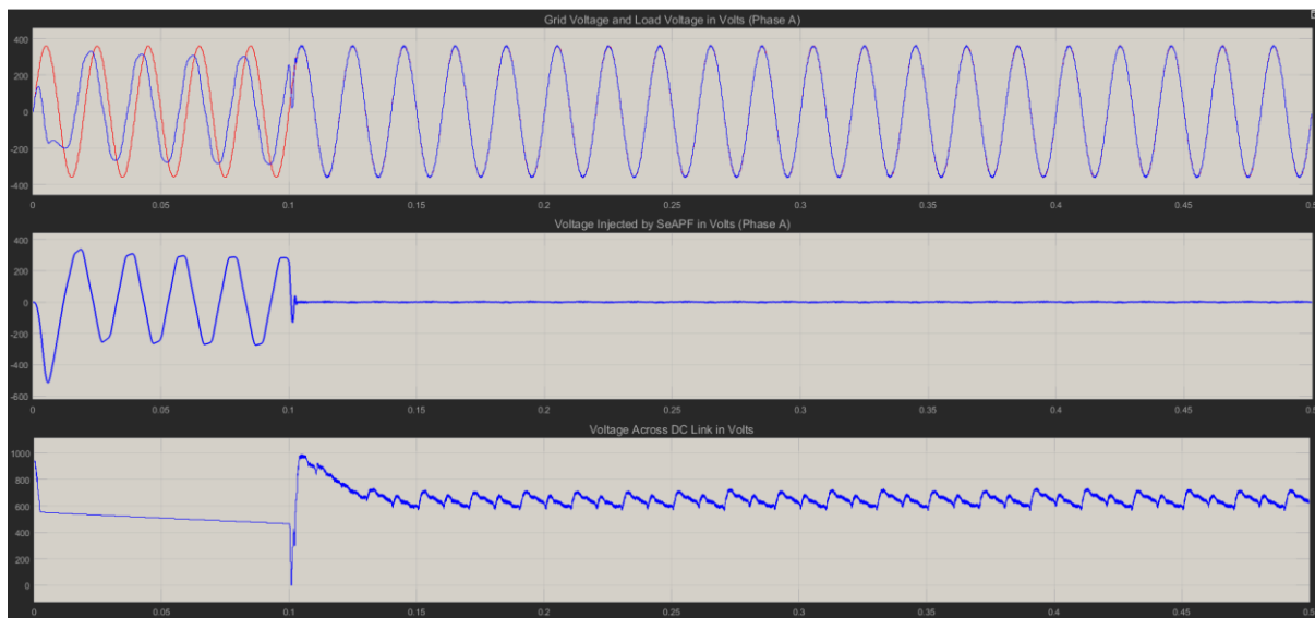
Fig8. Simulated waveforms of Series Active Filter (a) source voltage and Load Voltage. (b) Injected Voltage of the UPQC Voltage (c) Dc link Voltage.
