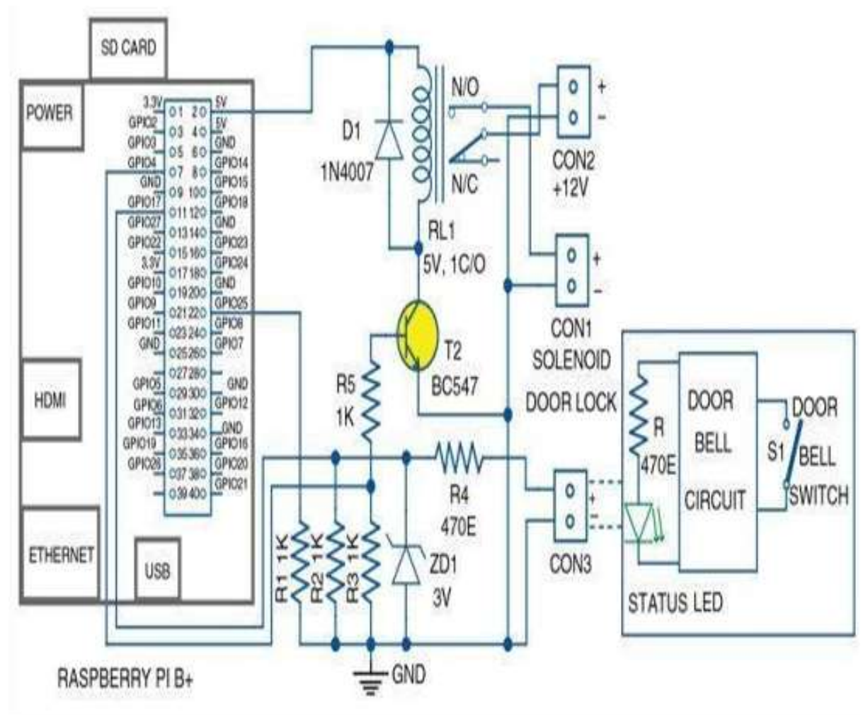
Fig 2: Circuit Diagram
