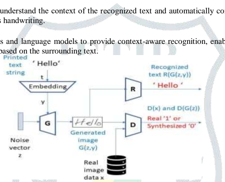
Figure 5 Handwriting image generation
