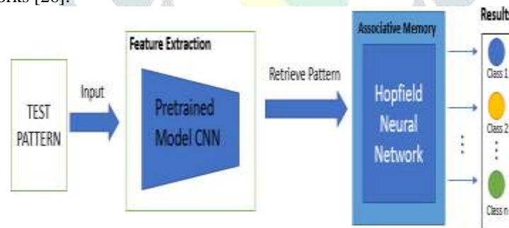
Figure 8 CNN-RNN hybrid model
