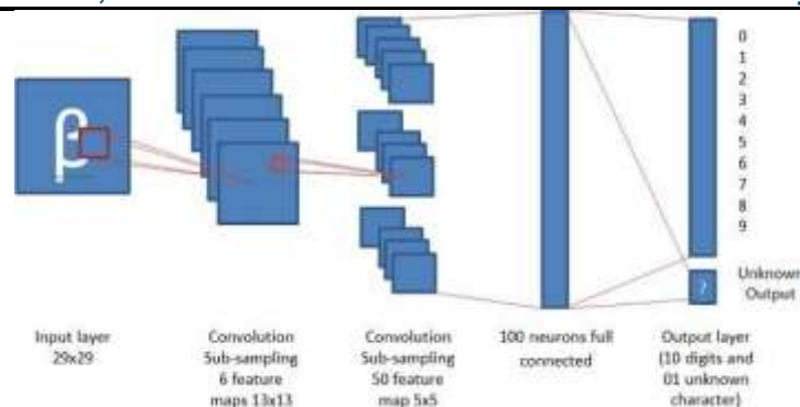
Figure 1 Introduction of Convolutional Neural Networks (CNNs)
