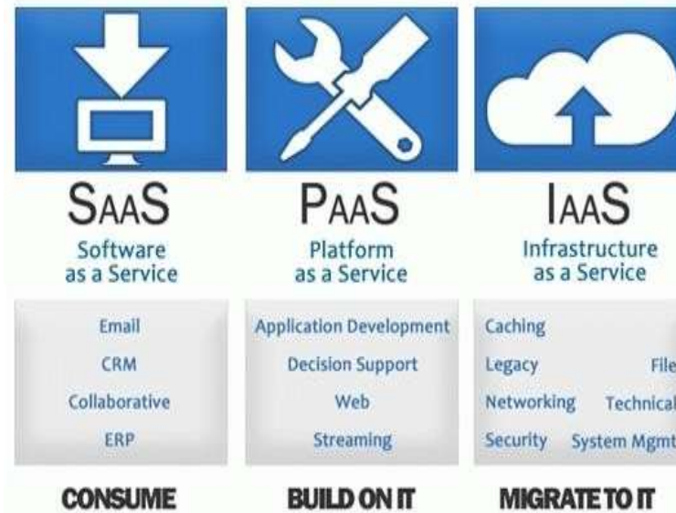
Fig.4 Cloud Services [8]
