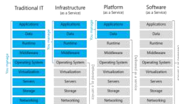
Figure 1: Distinct Cloud Models: Customer Managed versus Service Provider Managed
