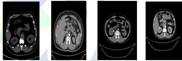
Figure 1. Sample Dataset
