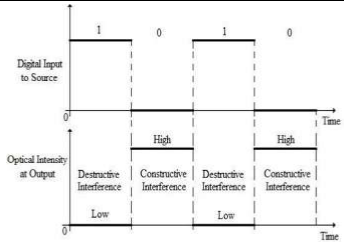
Fig. 3. Output of Mach Zehnder Interferometer to digital input at the source
