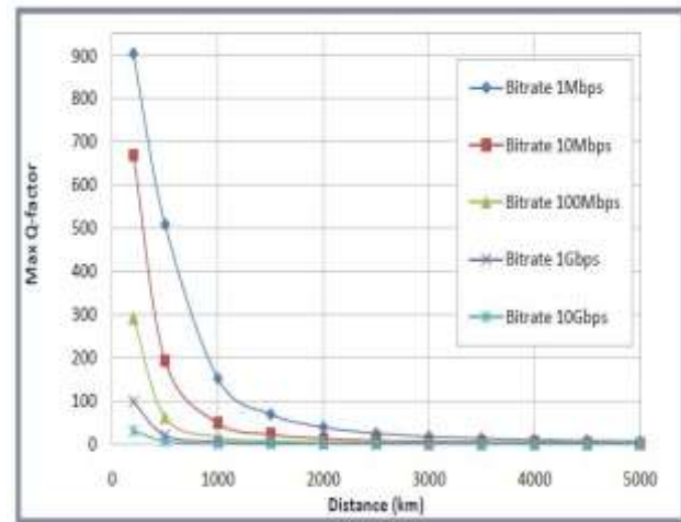
Fig. 6. Maximum achievable Q-factor for variable distance at 1550nm IsOWC link for bitrate up to 10Gbps
