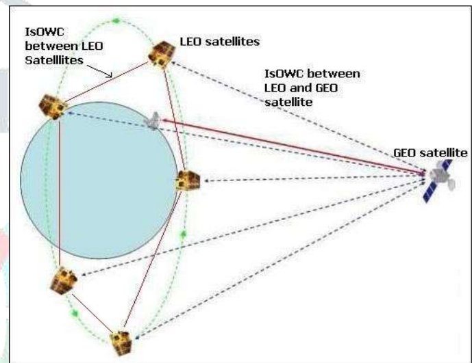
Fig. 1. Overview of IsOWC
