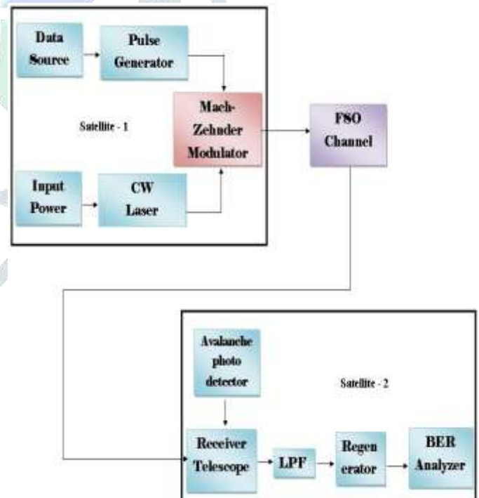
Fig. 4. Design of Inter Satellite Optical Wireless Communication System
