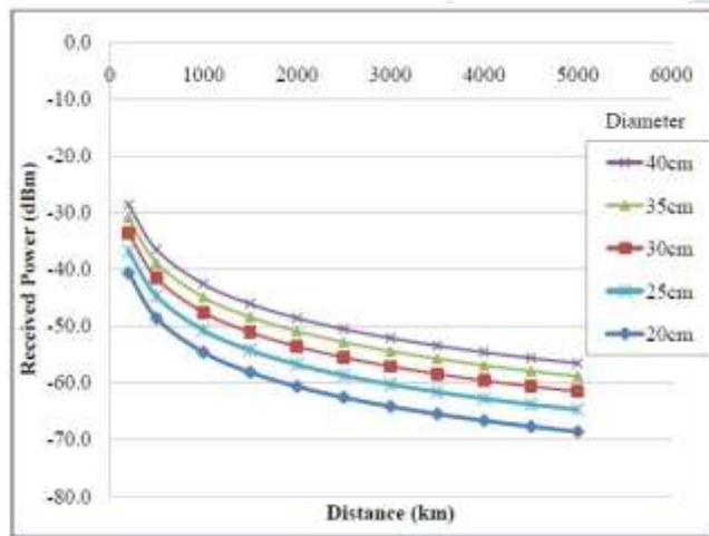
Fig. 7. Received power for respective optical antennae diameter at distance up to 5000km and input power of 10dBm.
