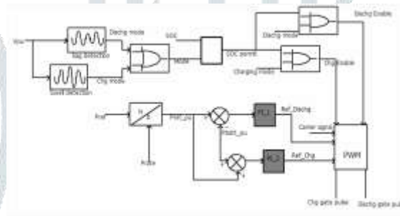
Fig 2: Control block diagram of BESS
