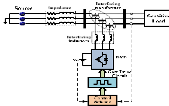
Fig 1: Schematic diagram of DVR connected in power system
