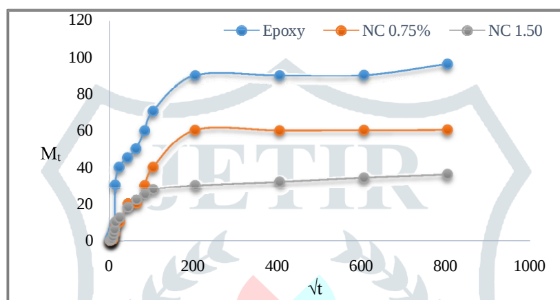
Figure 1. sorption kinetics of epoxy specimens for moisture absorption for the epoxy and the epoxy filled with 0.75 wt and 1.5 wt % of nanoparticles in an atmosphere with 91% during moisture absorption.
