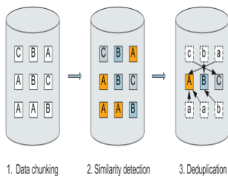
Fig 1: Process of De-Duplication
