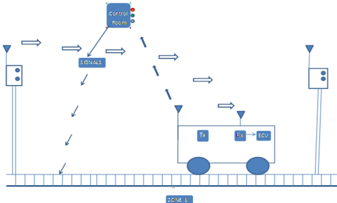
Fig:-.4.1 Main block diagram
