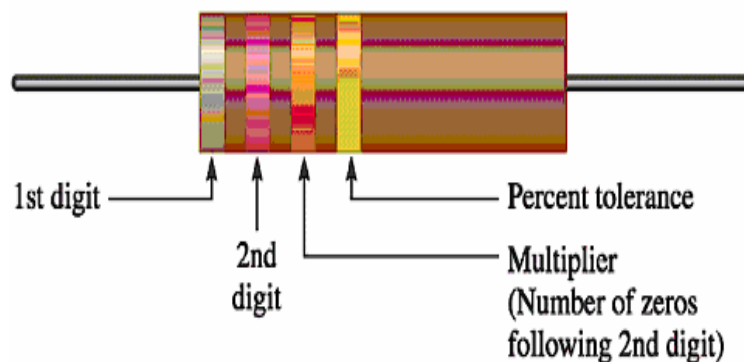
Fig 3.1.1 Resistor
