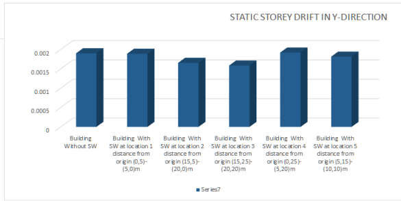
Static Storey Drift in Y-Direction (Unitless)
