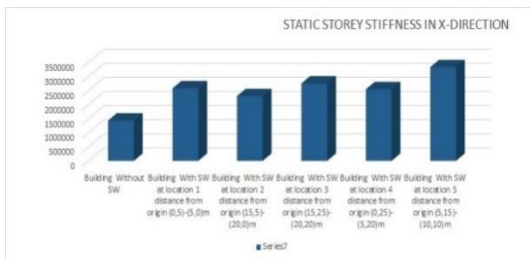
Static Storey Stiffness in X-Direction (KN/M)
