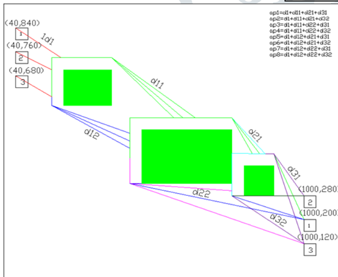
Figure 2 – Alternate paths of 3 robots with 3 obstacles.
