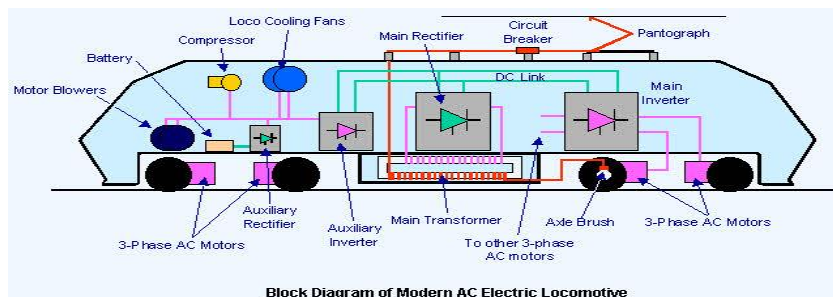
Fig.3 block diagram of modern ac electric locomotive
