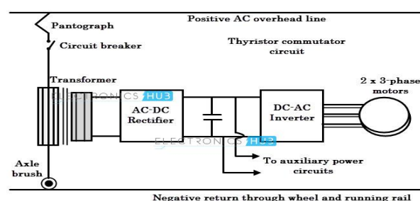
Fig.4 negative return through wheel and running rail
