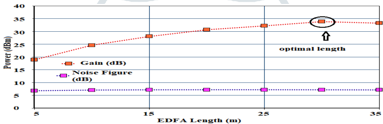
Figure 8 Effect of EDF lengths on Gain and noise figure of proposed L-band EDFA
