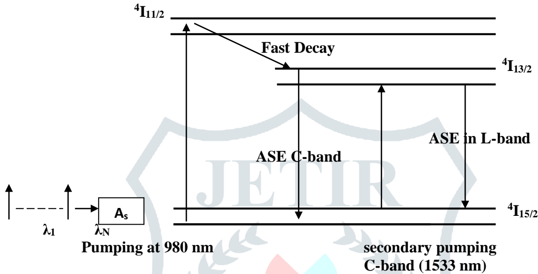
Figure 1 Principle of L-band EDFA ASE induced system employing FBGs ( Er^{3+} energy diagram)
