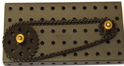
Figure 3 Chain Drive
