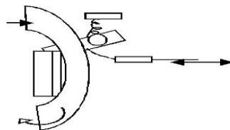
Figure 4. Braking system
