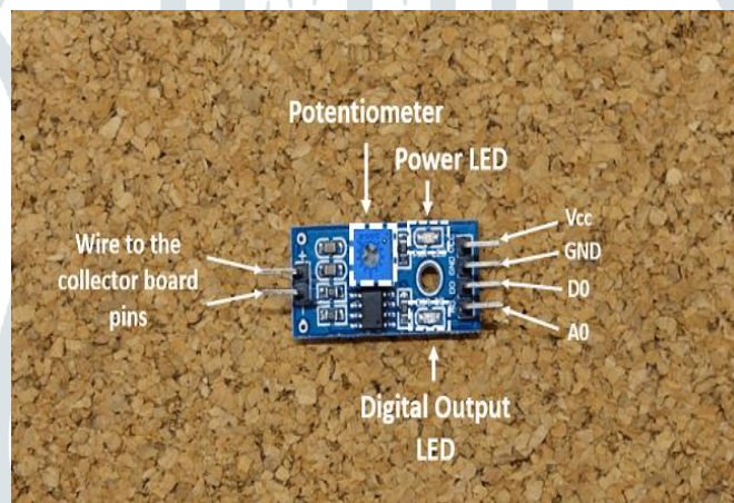
Fig 3: Soil Moisture Sensor Module.
