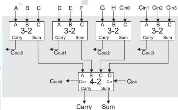
Fig. 6. Architecture 3 to implement 8:2 Adder compressor
