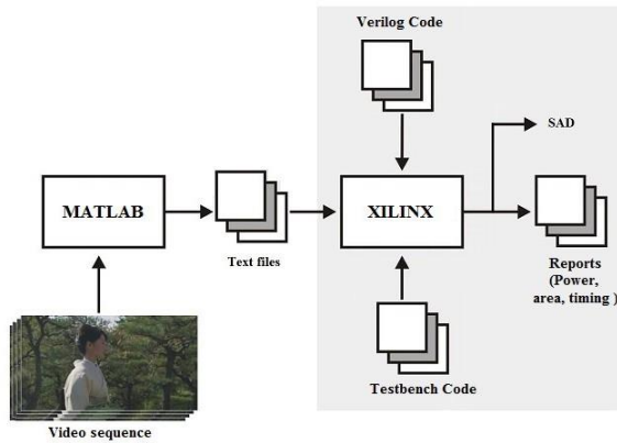
Fig. 10. Simulation workflow
