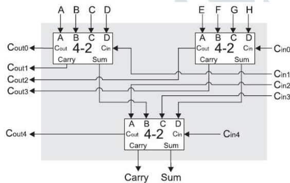
Fig. 4. Architecture 1 to implement 8:2 Adder compressor
