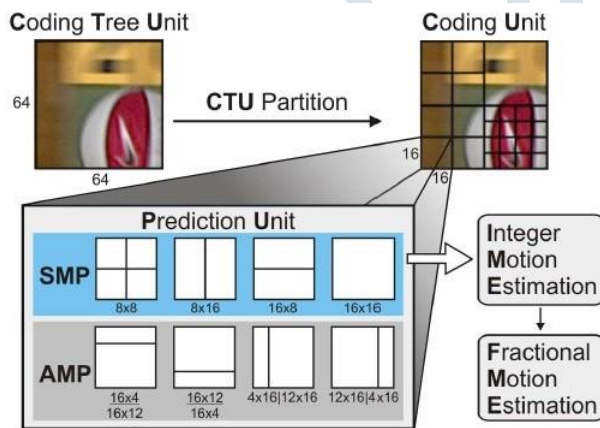
Fig. 8. Coding tree unit and the partitioning types.
