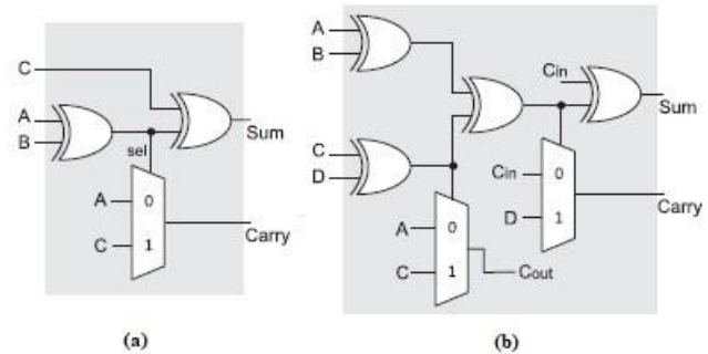
Fig. 1. Adder Compressors internal structures (a) 3-2; (b) 4-2.
