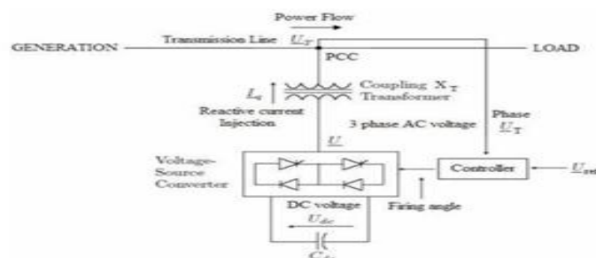
Fig. 4 STATCOM operation in a power system
