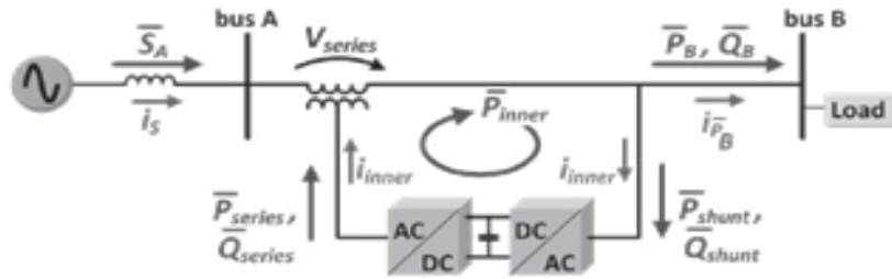
Fig. 6 UPQC power flow in steady state
