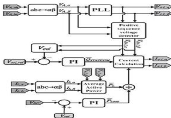
Fig. 5 Control algorithm of UPQC Controller
