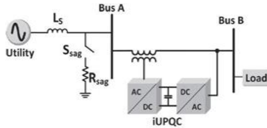
Fig. 7 UPQC experimental scheme
