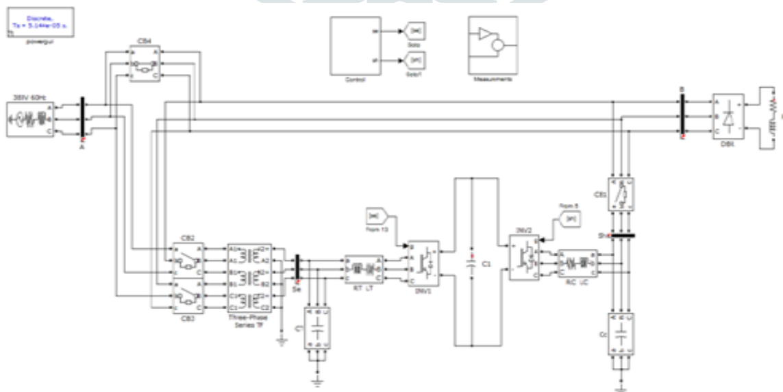
Fig. 8 Simulation circuit
