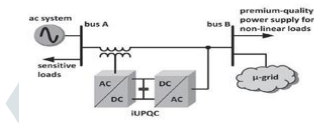
Fig. 1 General UPQC
