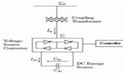
Fig. 3 Structure of a STATCOM
