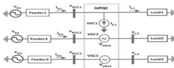
Fig. 2 System configuration of UPQC
