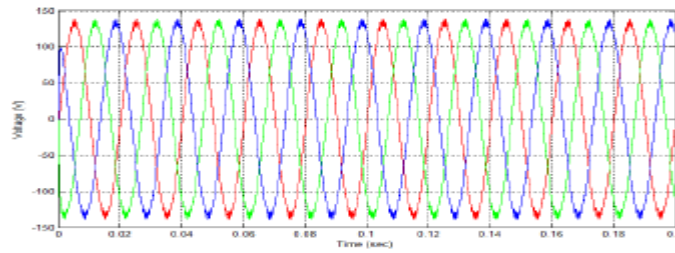
Fig.16. Sinusoidal output voltage waveform for three phase 11 level inverter using VF-PWM technique with series LC filter.
