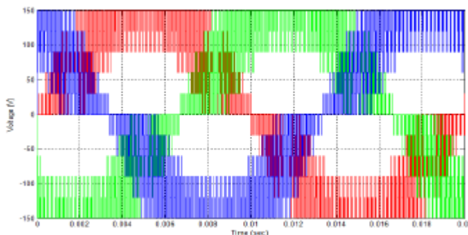
Fig.12. Output voltage waveform for three phase 11 level Inverter using CO-PWM technique.
