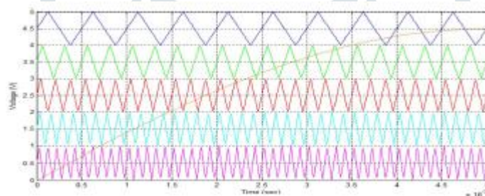
Fig.7. Reference Sine wave and Carrier waves for VF-PWM at m_a=0.9
