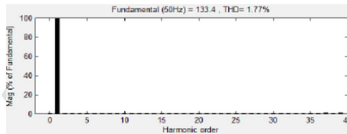
Fig.17. FFT Analysis of the harmonic spectrum for VF-PWM technique (with LC filter)
