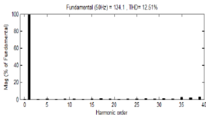
Fig.15. FFT Analysis of the harmonic spectrum for VF-PWM technique
