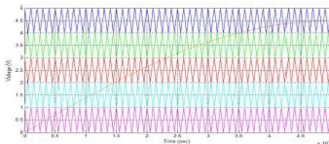
Fig.5. Reference Sine wave and Carrier waves for APD-LSPWM at m_a=0.9 and m_f=200 .
