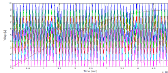
Fig.6. Reference Sine wave and Carrier waves for COPWM method at m_a=0.9 and m_f=200 .
