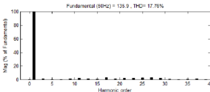
Fig.11. FFT Analysis of the harmonic spectrum for APD-LSPWM technique
