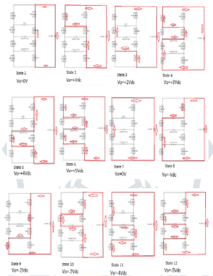
Fig.3. States corresponding to each Output voltage level
