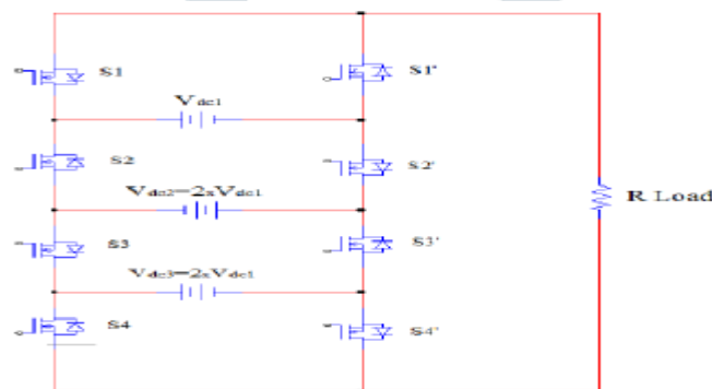
Fig.1. Proposed configuration for single phase inverter operation
