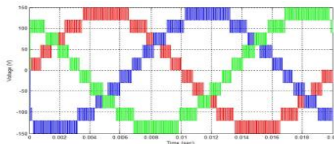
Fig.8. Output voltage waveJorm Jor three phase II level inverter using iPDLSPWM technique.
