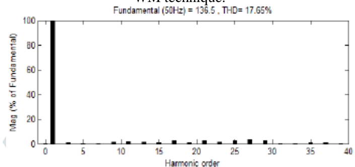
Fig.9. FFT Analysis of the harmonic spectrum for iPD-LSPWM technique
