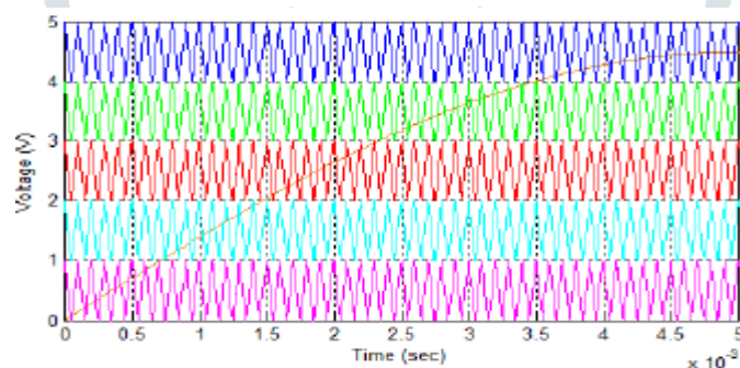
Fig.4. Reference Sine wave and Carrier waves for JPD-LSPWM at m_a=0.9 and m_f=200 .
