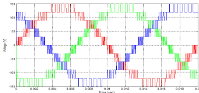
Fig.14. Output voltage waveform for three phase 11 level Inverter using VF-PWM technique.
