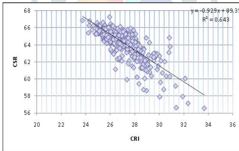
Figure 3: Graph between CSR and CRI
