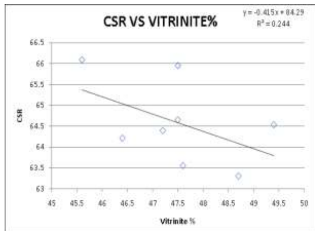
Figure 1: Graph between CSR and Vitrinite %
