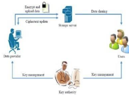
Fig. 1. A natural RIBE-based data sharing system
