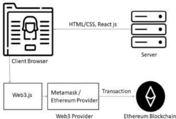
Figure 3: System Architecture [19].
