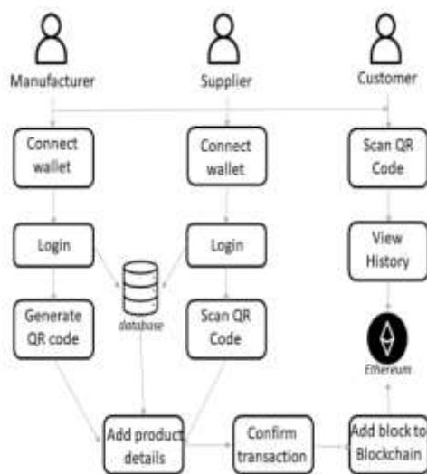
Figure 4: System Flow.
